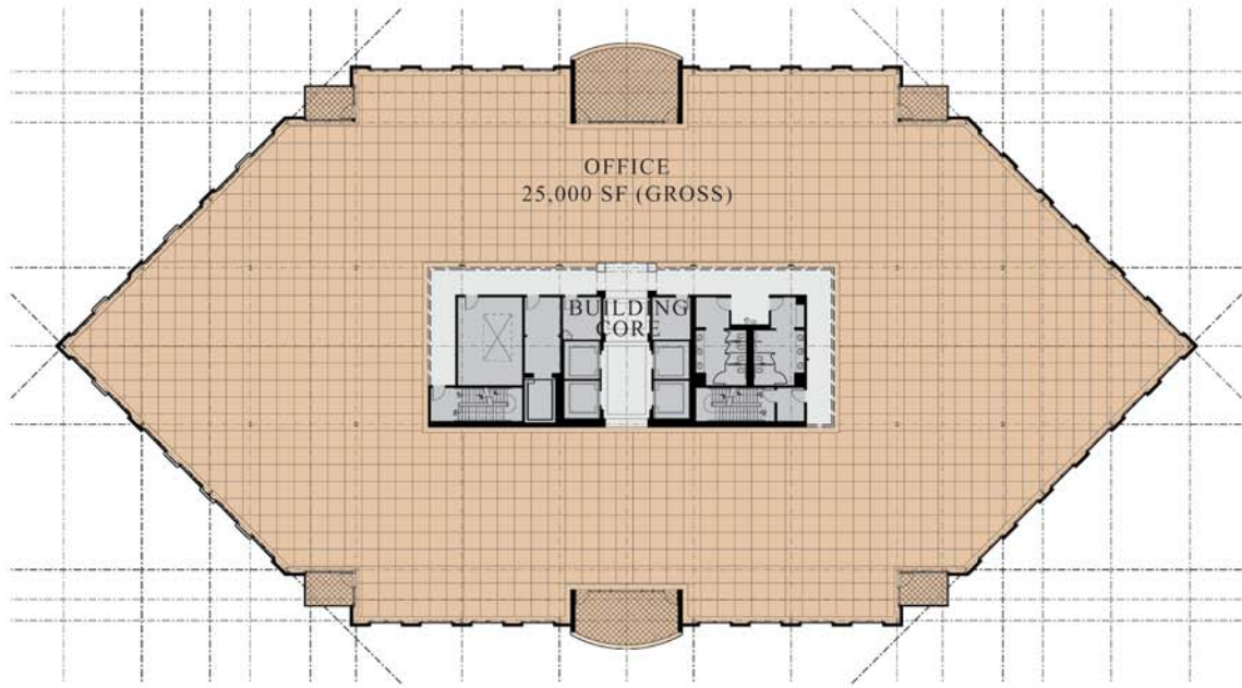
EIGHTH LEVEL FLOOR PLAN
