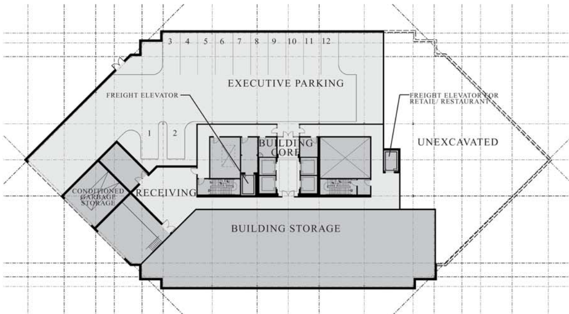
LOWER LEVEL FLOOR PLAN
